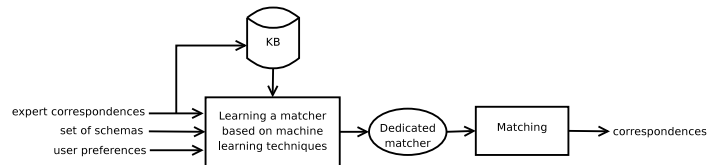
Figure 1: YAM Architecture
